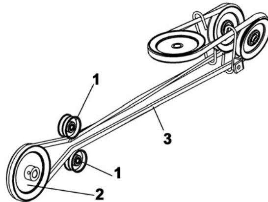
Install belt
